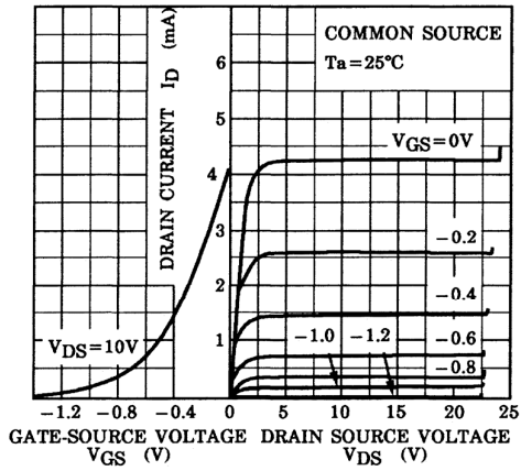
STATIC CHARACTERISTICS
