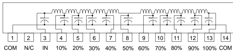
10-Tap SIP5 Style Schematic
