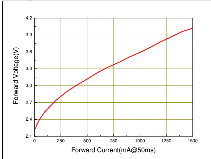
Forward Voltage vs Forward Current, T_{\text{solder pad}} = 25^{\circ}\text{C}
