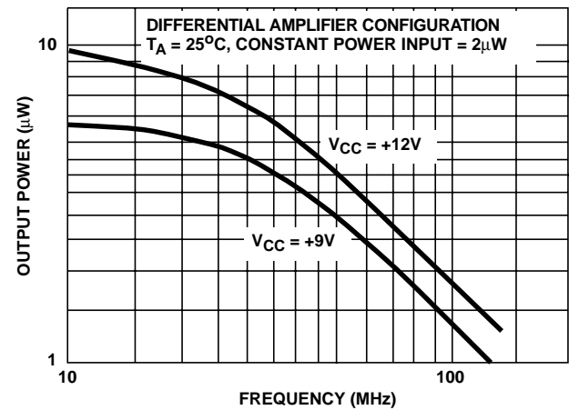
FIGURE 28. OUTPUT POWER vs FREQUENCY - 50Ω INPUT AND 50Ω OUTPUT (DIFFERENTIAL AMPLIFIER CONFIGURATION)
