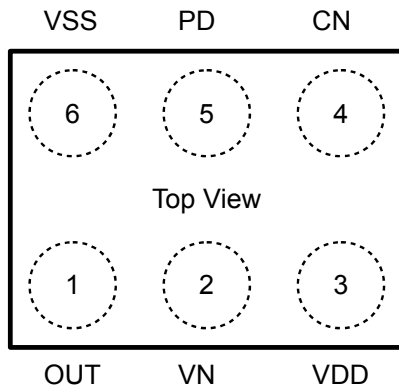
6-Pin Chip Scale Package (CSP)
