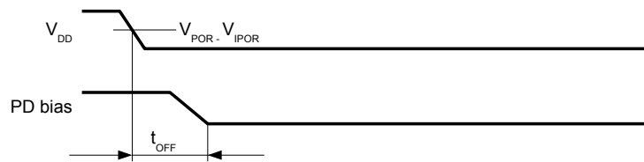
Power-down sequence
