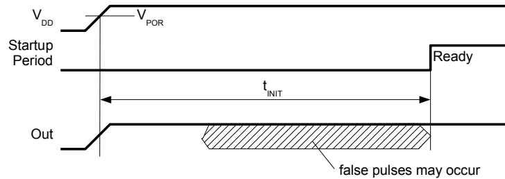
Power-up sequence
