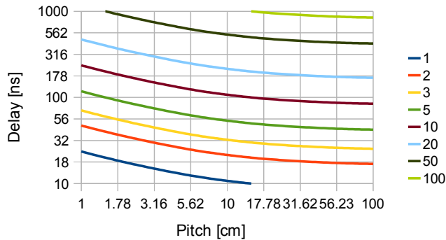
Figure 10: Delay vs Pitch. Parameter: Line length [m]
