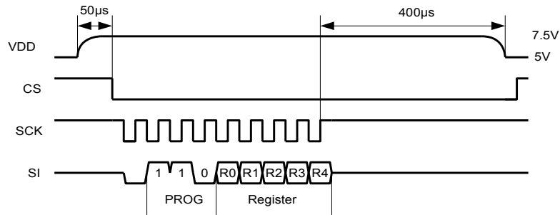
Figure 21: Direct programming procedure
