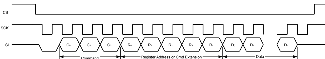
Figure 17: Communication to the interface device (Direct Command)
