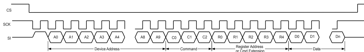
Figure 18: Communication to the sensor devices (Broadcast Command)
