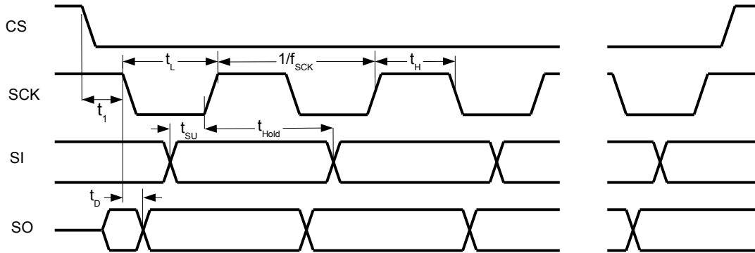
Figure 16: SPI bus timing
