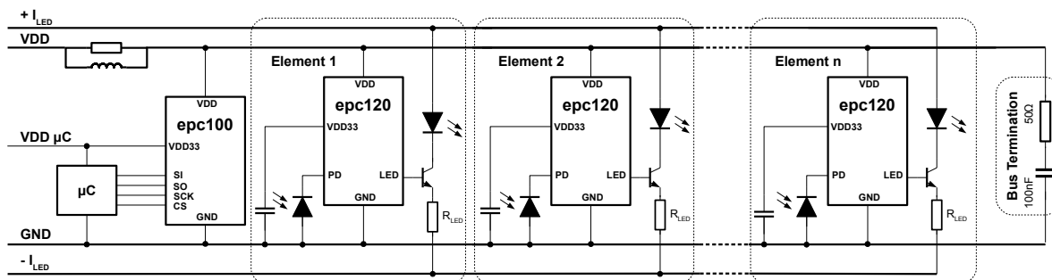
Figure 5: epc120 in the light barrier application as receivers and the interface chip to the microcontroller
