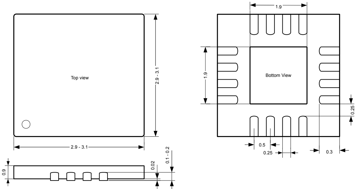
Figure 25: QFN-16: Mechanical dimensions
