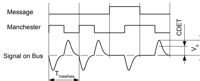
Figure 11: Manchester encoded signal on the bus
