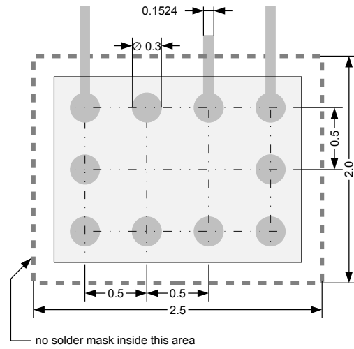
Figure 24: CSP10: Layout recommendation
