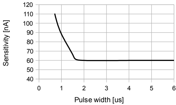
Figure 1: Input Sensitivity vs. LED pulse width
