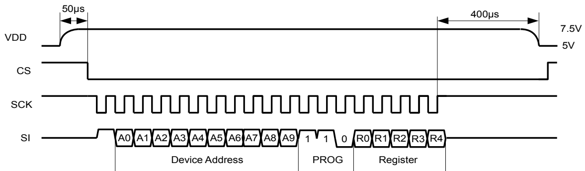
Figure 22: Broadcast programming procedure
