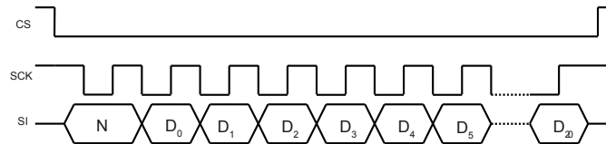
Figure 20: Timing Result Data
