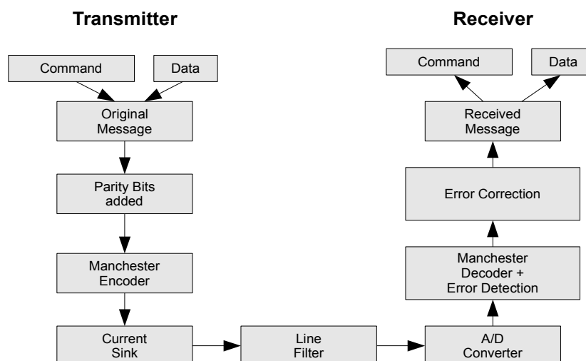
Figure 6: Data handling
