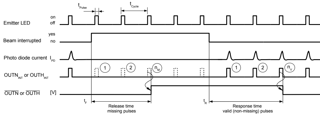
Figure 6: Pulse modulation concept
