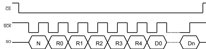
Figure 16: Timing Result Data
