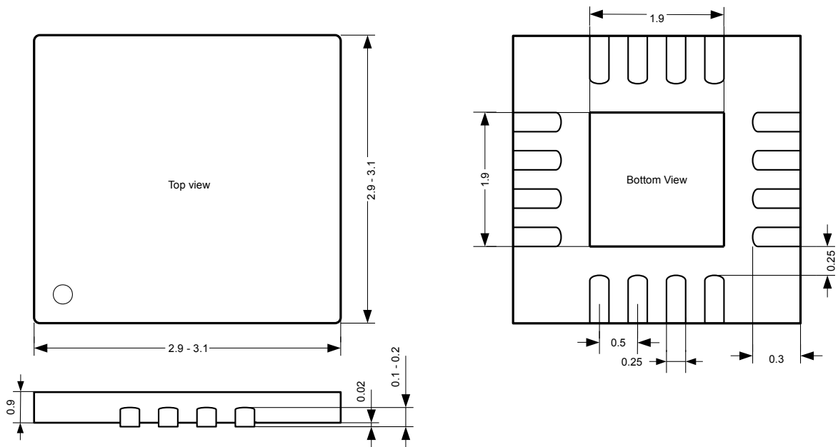
Figure 26: QFN-16: Mechanical dimensions
