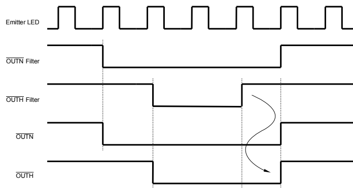
Figure 7: synchronization \overline{OUTH} with \overline{OUTN}
