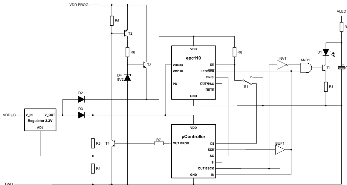
Figure 13: Hardware interface micro-controller – epc110
