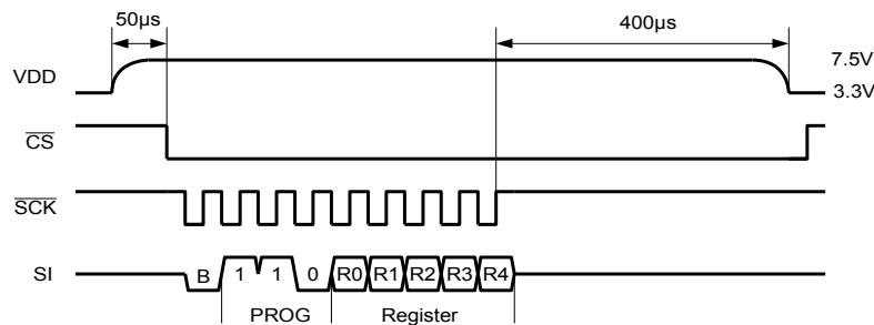
Figure 17: Direct programming procedure
