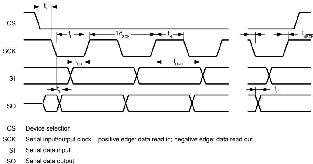
Figure 14: SPI bus timing
