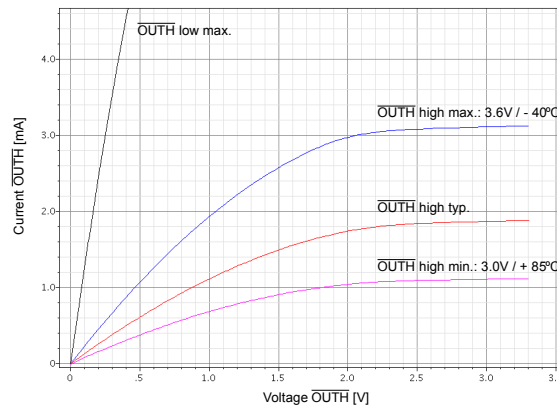
Figure 8: Output voltage versus output current of output \overline{OUTH}
