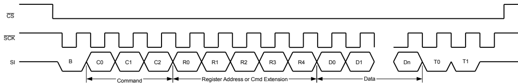
Figure 15: Communication to the epc110 device: Direct Command
