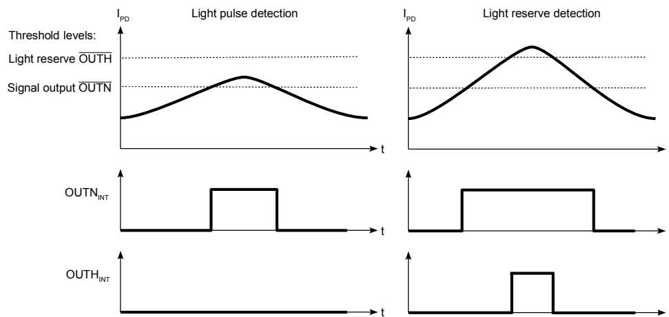
Figure 5: Pulse evaluation
