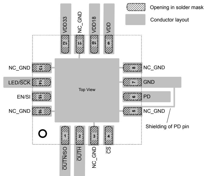
Figure 25: QFN-16: Layout recommendation
