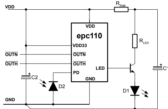
Figure 3: Principle of standalone light barrier application
