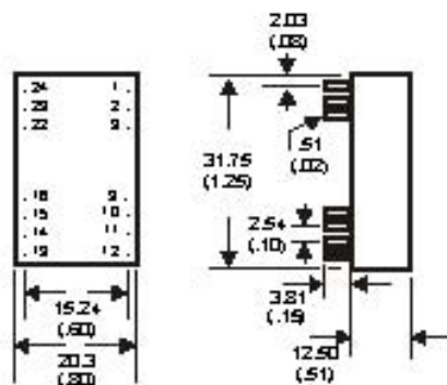
DIMENSIONS: BOTTOM VIEW
