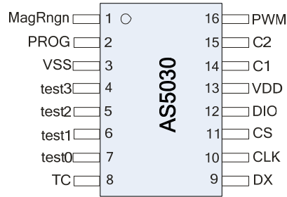
Figure 3: TSSOP-16 package and pin-out
