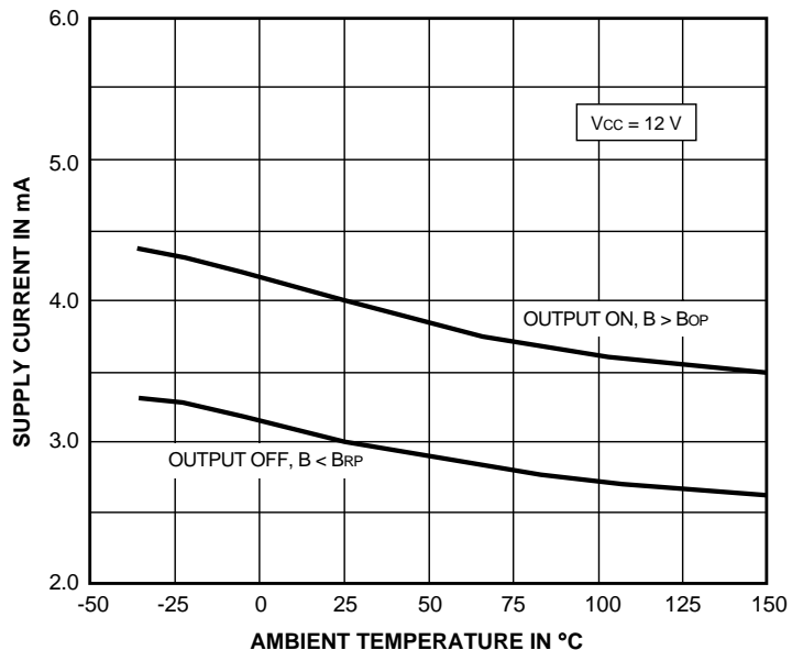
SUPPLY CURRENT
