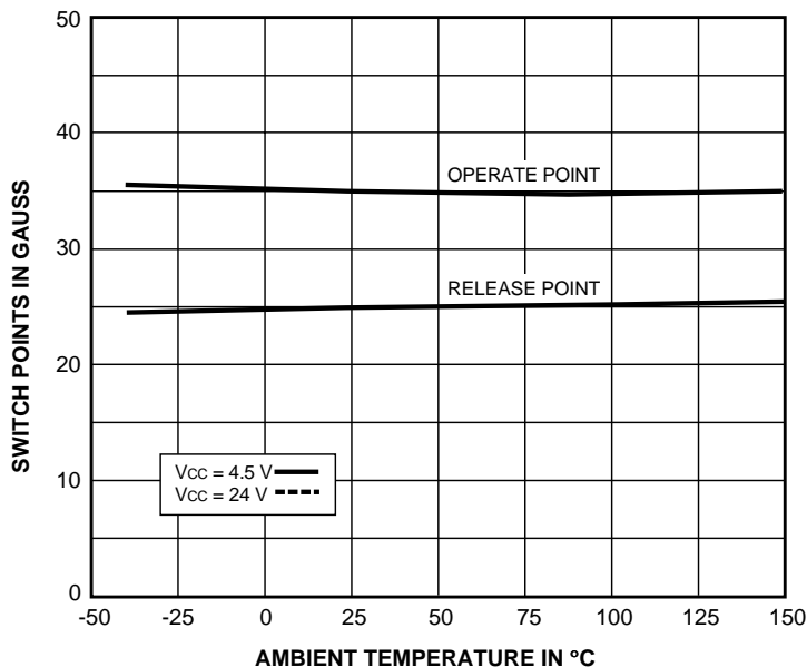
SWITCH POINTS
