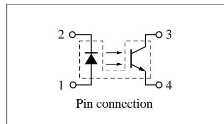
Internal connector
