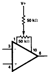
Voltage Offset Null Circuit (Note 1)
