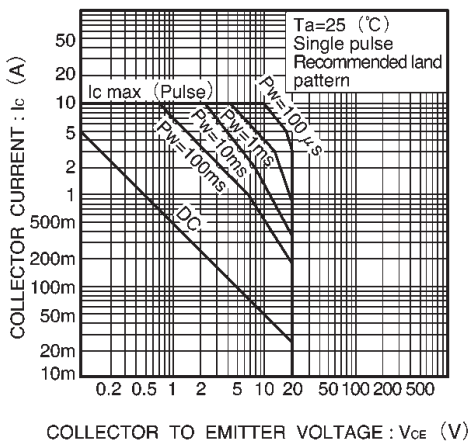
Fig.13 Safe operating area (2SD2098)
