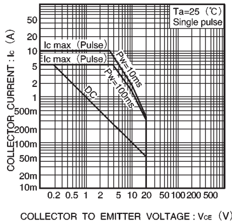
Fig.14 Safe operating area (2SD2118)
