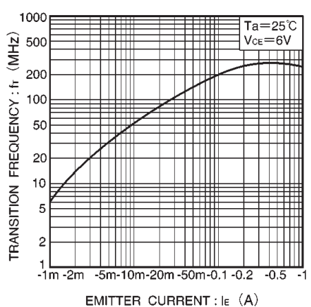
Fig.11 Gain bandwidth product vs. emitter current
