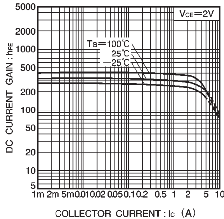
Fig.5 DC current gain vs. collector current ( III )
