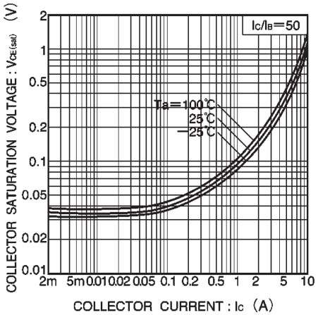
Fig.10 Collector-emitter saturation voltage vs. collector current (V)
