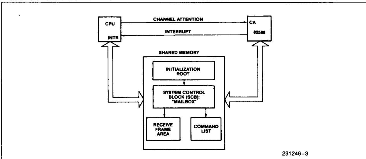
Figure 3. 82586/Host CPU Interaction
