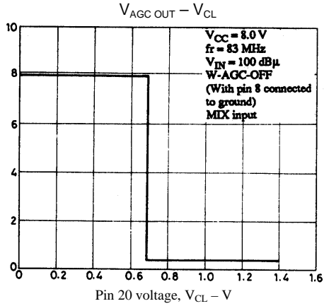
Pin 16 AGC output voltage - V
