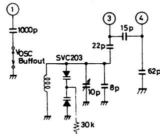
Unit (Resistance: \Omega , Capacitance: F)
