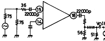
Unit (Resistance: \Omega , Capacitance: F)
