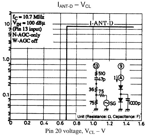
Antenna damping current - mA
