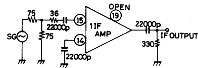
Unit (Resistance: Ω, Capacitance: F)
