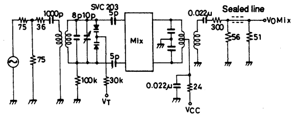
Unit (Resistance: Ω, Capacitance: F)
