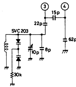
Unit (Resistance: \Omega , Capacitance: F)
