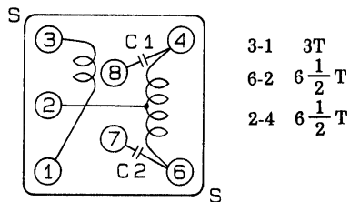
Mixer coil (for both bands) SA-266
