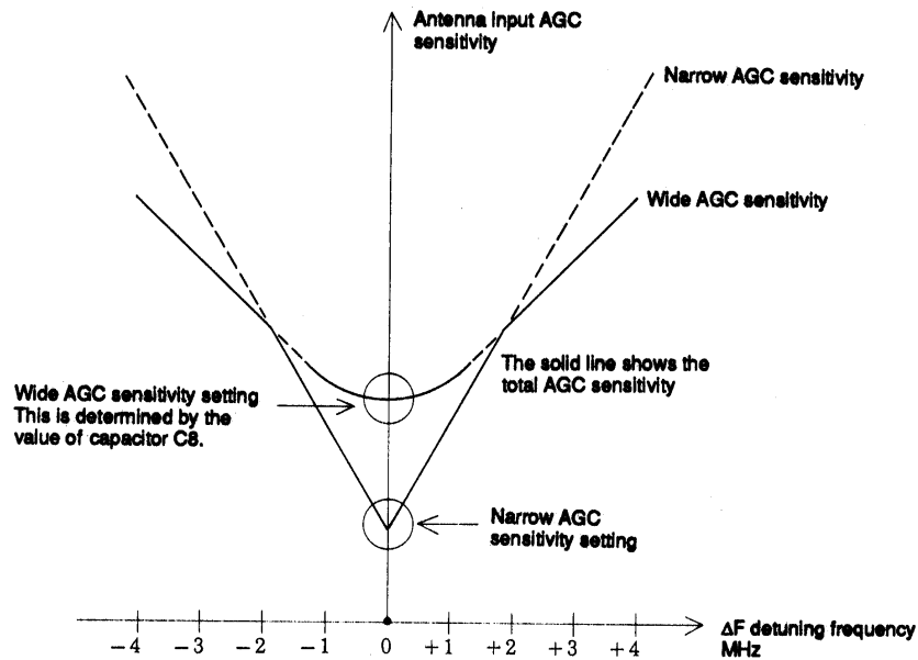
Figure 2 AGC Sensitivity Detuning Characteristics
