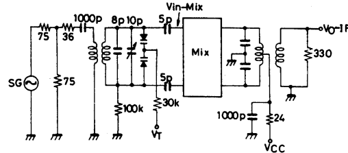
Unit (Resistance: Ω, Capacitance: F)
