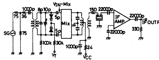
Unit (Resistance: \Omega , Capacitance: F)
