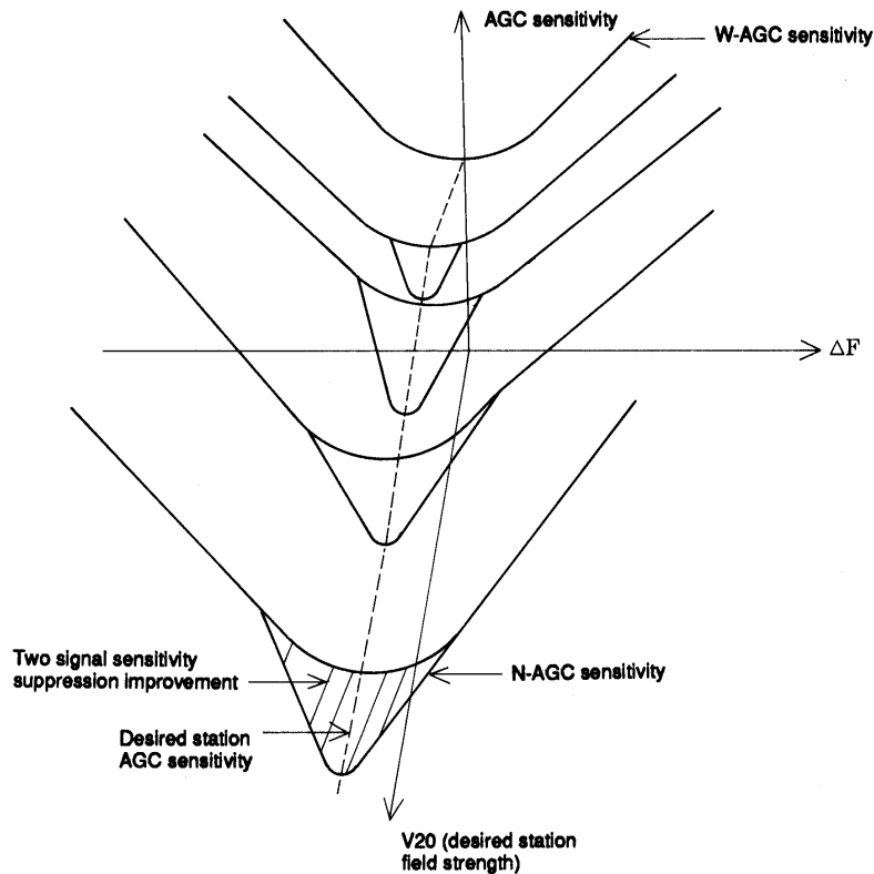
Figure 3 3D-AGC Sensitivity, \Delta f and V_{20} Characteristics
