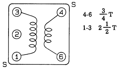
US band antenna coil SA-140 or SA-231
