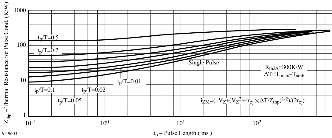
Figure 10. Thermal Response
