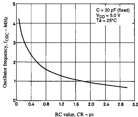
Fig. 2 Oscillator Frequency
