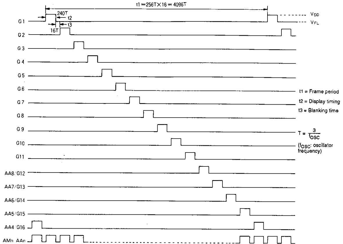
Fig. 3 Grid Timing Chart (16 display digits)
