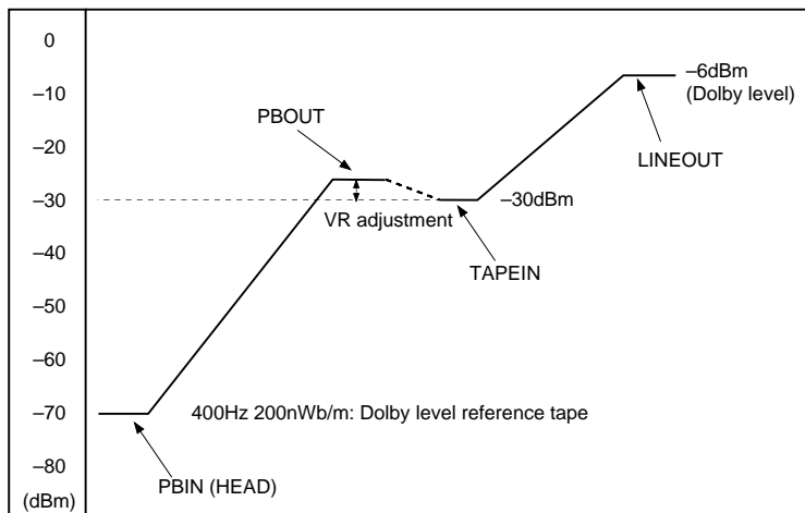
Fig. 2. Level diagram
