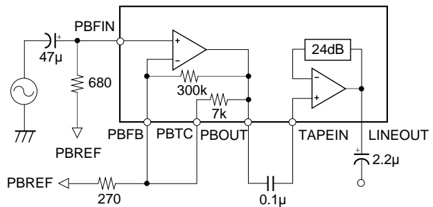
Fig. 7 Measurement circuit for crosstalk between channels
