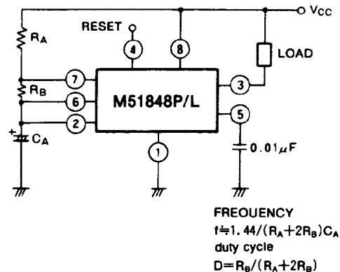
(2) Pulse oscillator (astable multivibrator)
