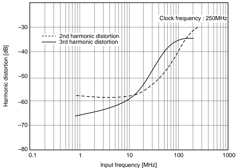
Harmonic distortion vs. Input frequency response characteristics
