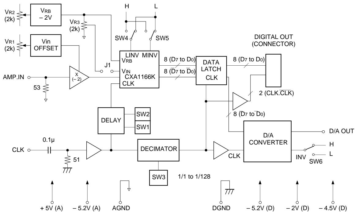
Fig. 1. Block Diagram
