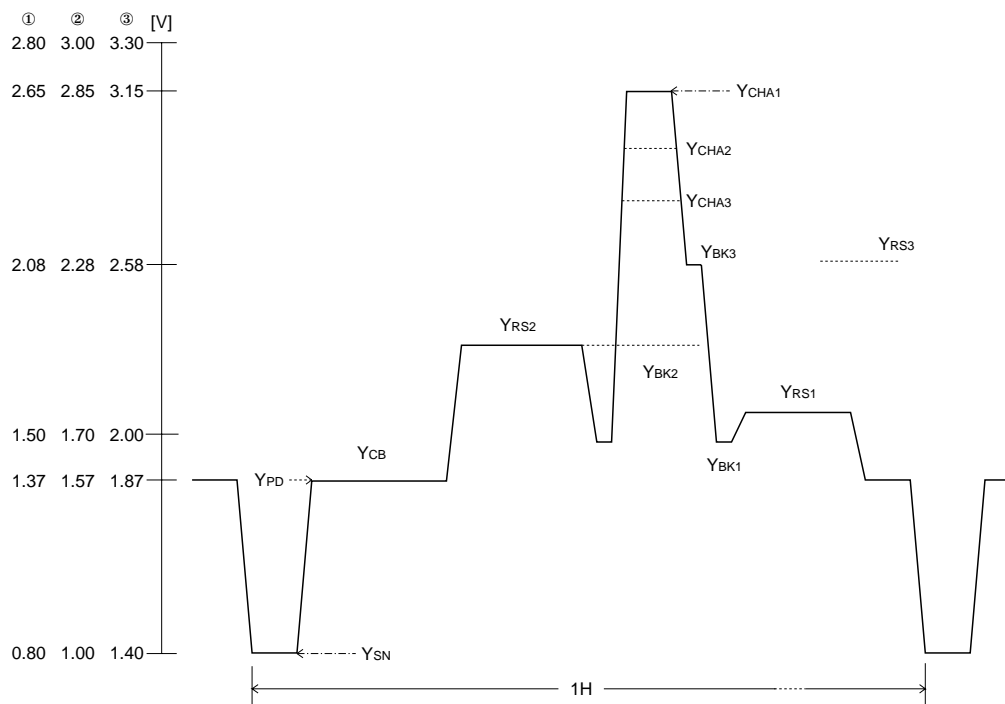
YOUT Output Level Waveform ( V_{DD2} = 5.00\text{ V} )
