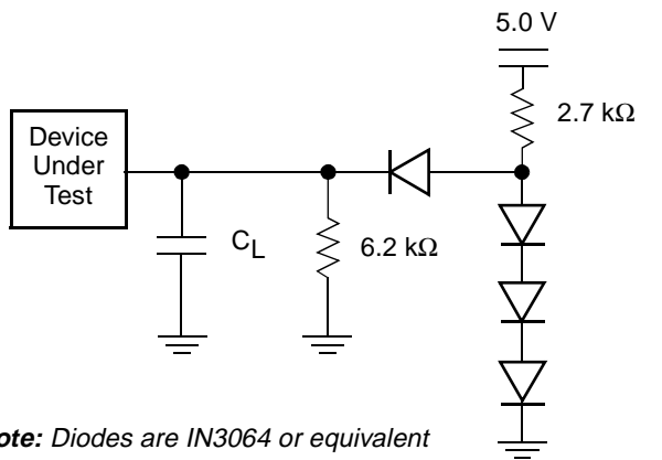
Figure 8. Test Setup
