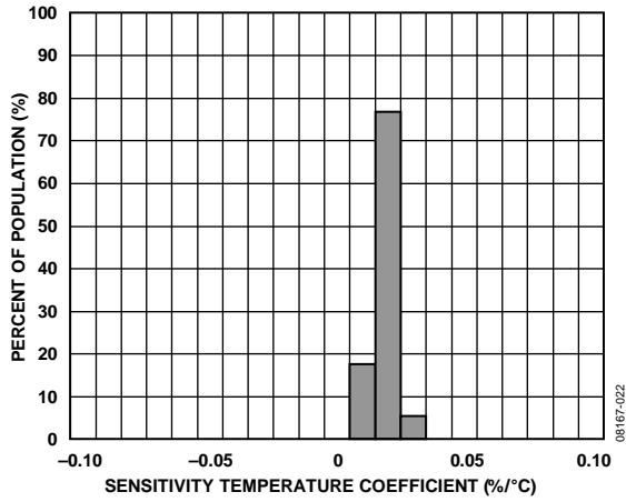
Figure 22. X-Axis Sensitivity Temperature Coefficient, V_S = 2.6\text{ V}
