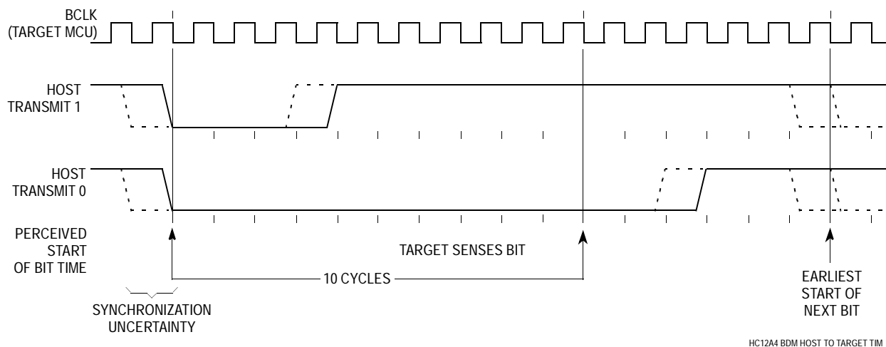
Figure 59 BDM Host to Target Serial Bit Timing
