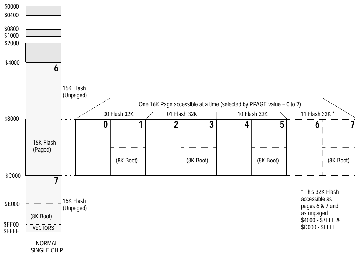
Figure 11 MC68HC912DT128A Memory Paging
