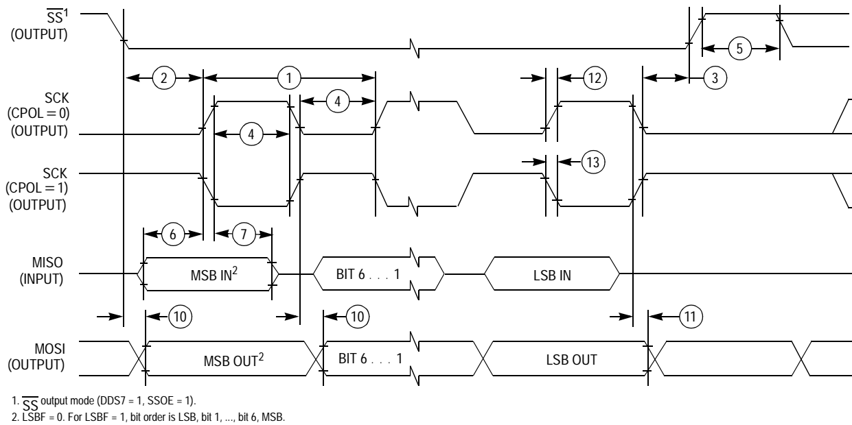
A) SPI Master Timing (CPHA = 0)
