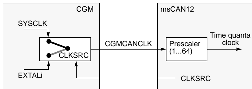
Figure 47 Clocking Scheme
