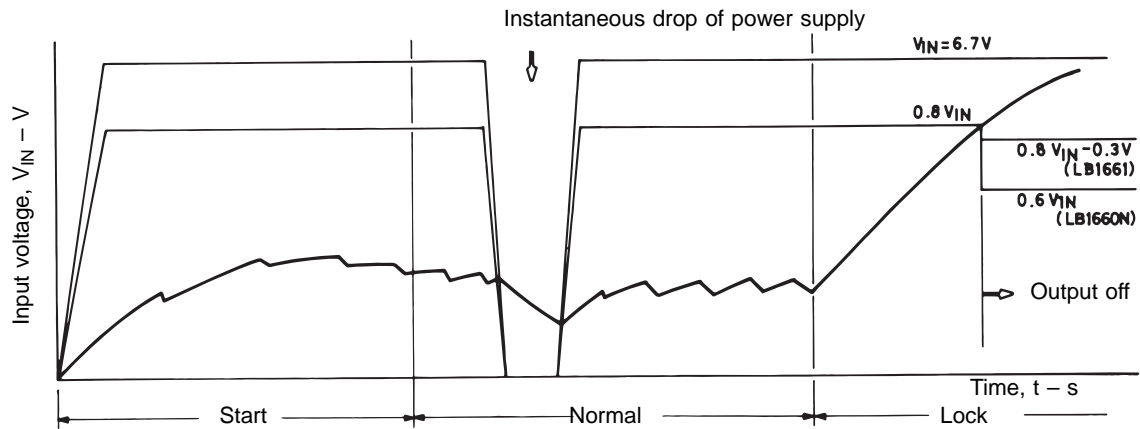
Timing Chart
