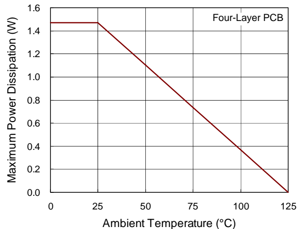
Figure 3. Derating Curves for RT9519A Package
