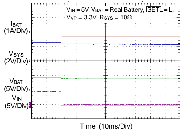
V_{IN} Removal
