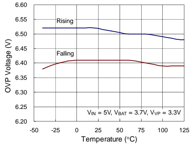
OVP Threshold Voltage vs. Temperature
