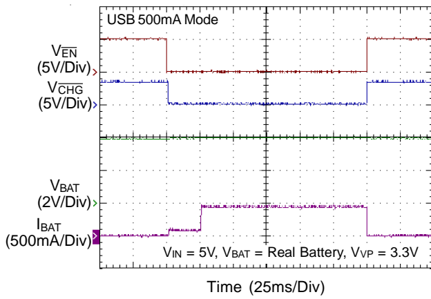
Charger On/Off Control from \overline{EN}
