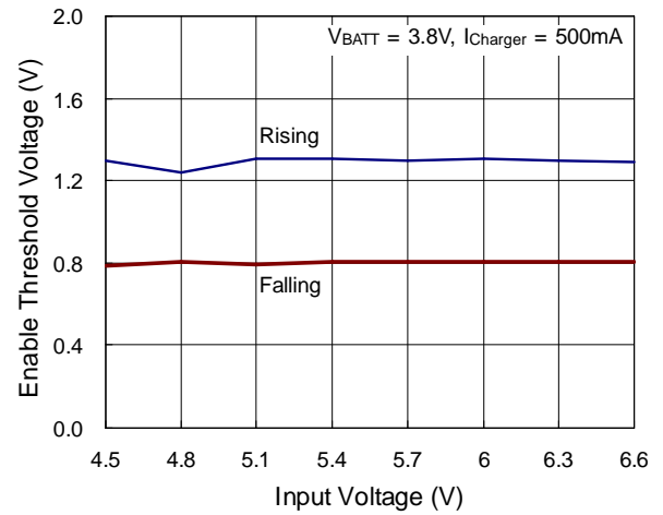
Enable Threshold Voltage vs. Input Voltage
