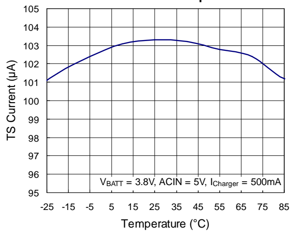
TS Current vs. Temperature
