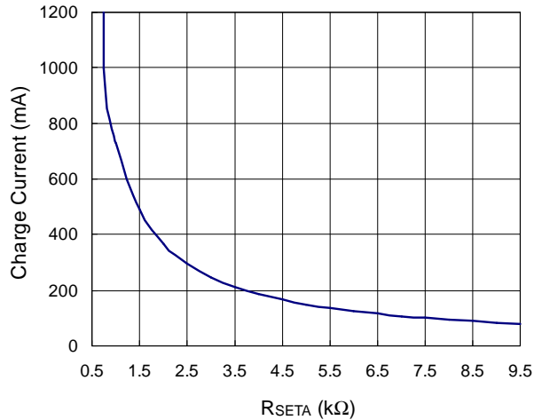
Figure 7. ACIN Mode Charge Current Setting
