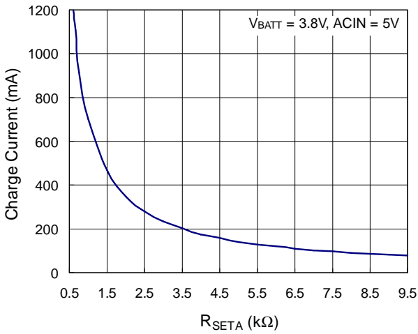
Charge Current vs. R SETA
