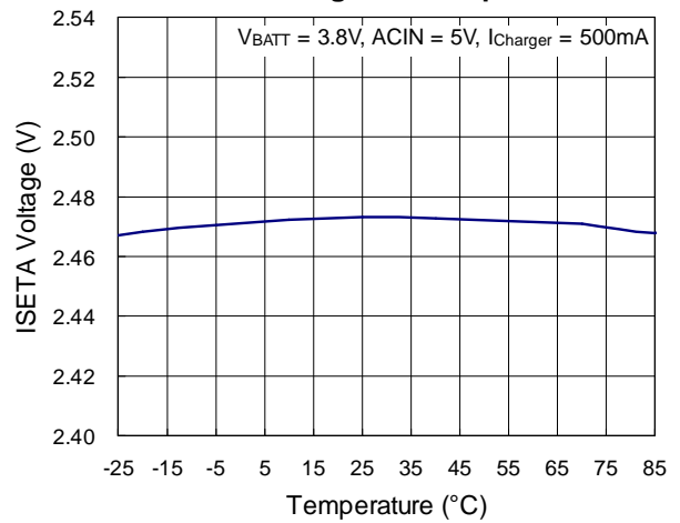
ISETA Voltage vs. Temperature
