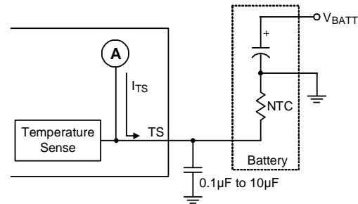
Figure 5. Temperature Sensing Configuration
