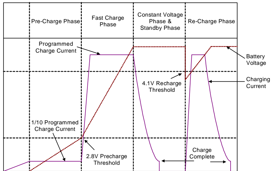
Figure 1 . Charging I-V Curve
