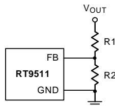
Figure 8. Setting the Output Voltage
