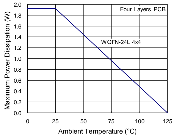
Figure 9. Derating Curves for RT9511 Packages
