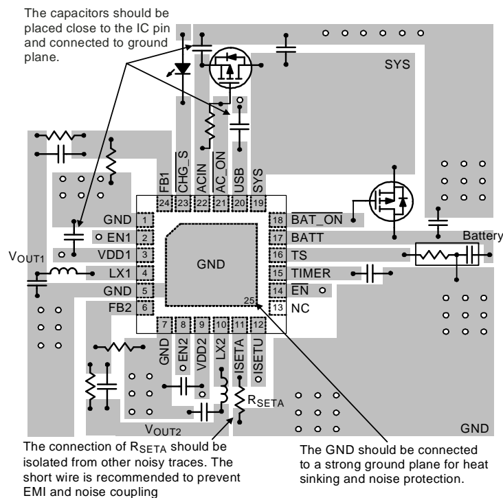
Figure 10. PCB Layout Guide
