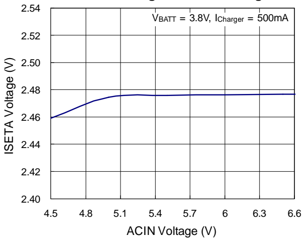
ISETA Voltage vs. ACIN Voltage
