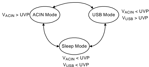
Figure 2. Input Power Source Operation Mode.
