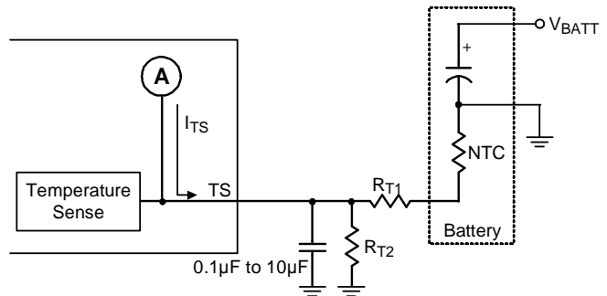
Figure 5. Temperature Sensing Configuration
