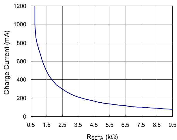
Figure 4. ACIN Mode Charge Current Setting
