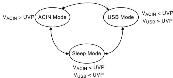
Figure 1. Input Power Source Operation Mode.
