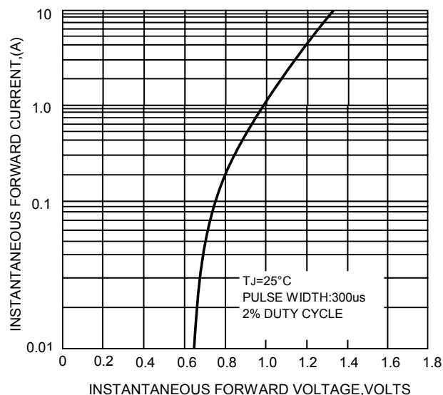
FIG.4-TYPICAL FORWARD CHARACTERISTICS
