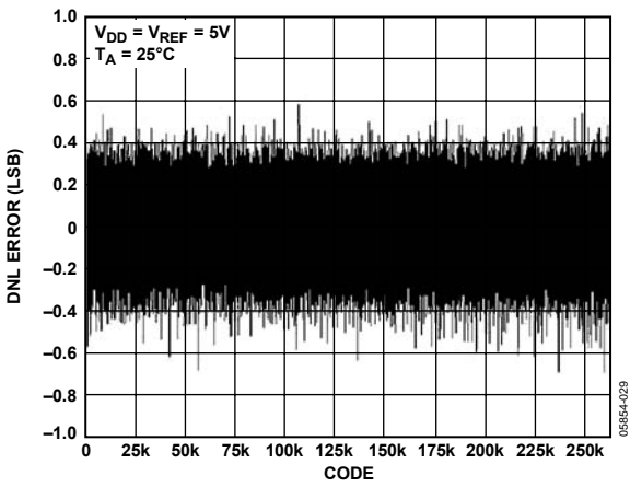
Figure 5. Typical DNL Plot in 50 Hz System Bandwidth
