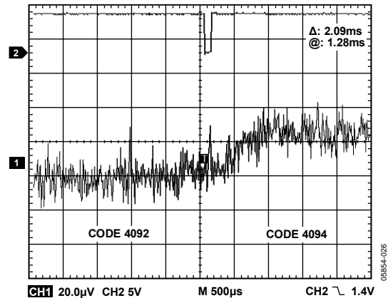
Figure 34. DAC Output with 300 Hz Filter on Output
