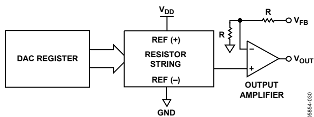
Figure 22. DAC Architecture
