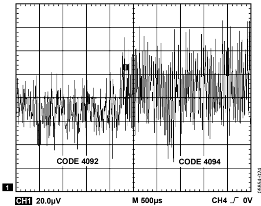
Figure 32. DAC Output Unfiltered
