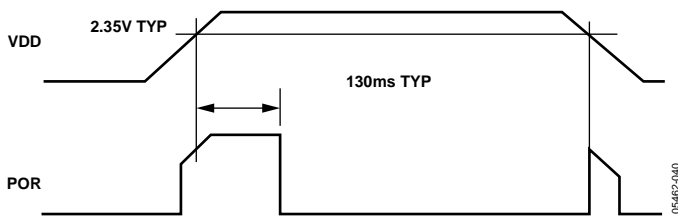
Figure 40. Internal Power-On Reset Operation
