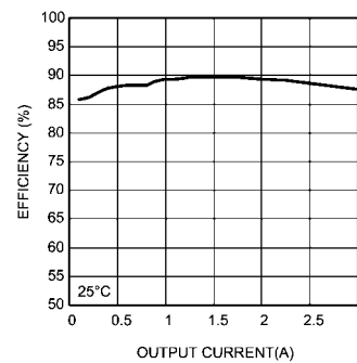
Efficiency V_{IN} = 24V V_{OUT} = 5.0V
