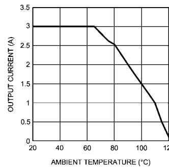
Thermal derating curve V_{IN} = 24V , V_{OUT} = 5.0V ,
