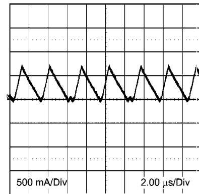
Transition Mode Operation V_{IN} = 24V, V_O = 3.3V, I_O = 0.29A
