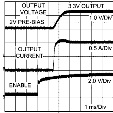
Pre-Biased Startup
