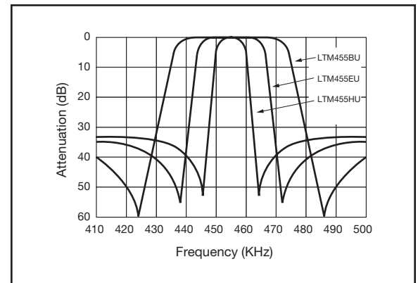
Figure 3) LTM450U – Characteristics
