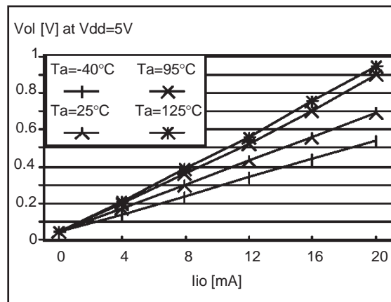
Figure 64. Typical V_{OL} at V_{DD} = 5V (high-sink)
