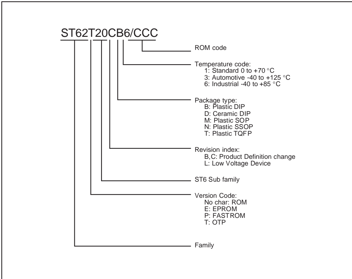
Figure 4. ST6 Factory Coded Device Types
