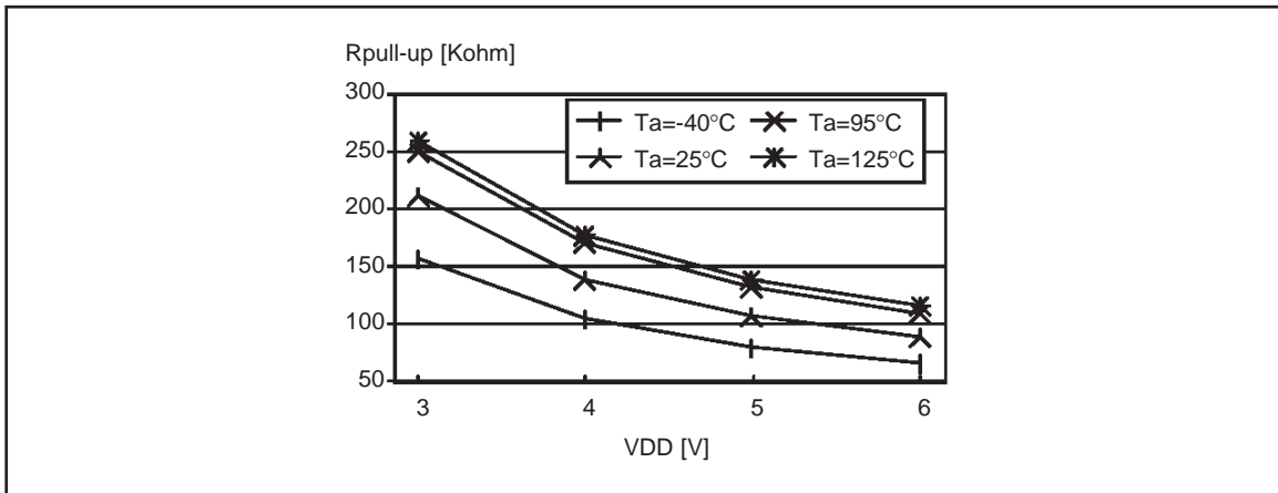
Figure 71. Typical R_{\text{pull-up}} vs. V_{\text{DD}} with V_{\text{IN}}=V_{\text{SS}}
