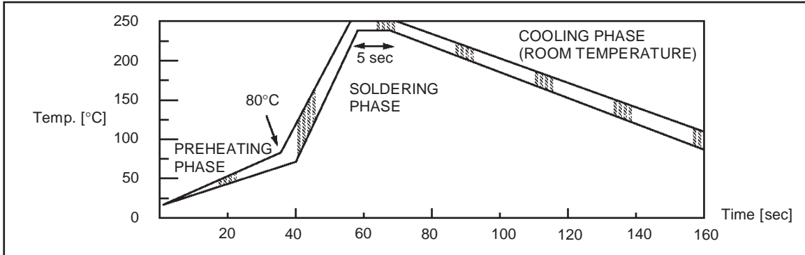
Figure 3. Recommended Reflow Soldering Oven Profile (MID JEDEC)
