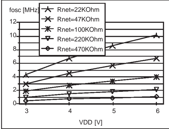
Figure 52. Typical RC Oscillator frequency vs. R NET
