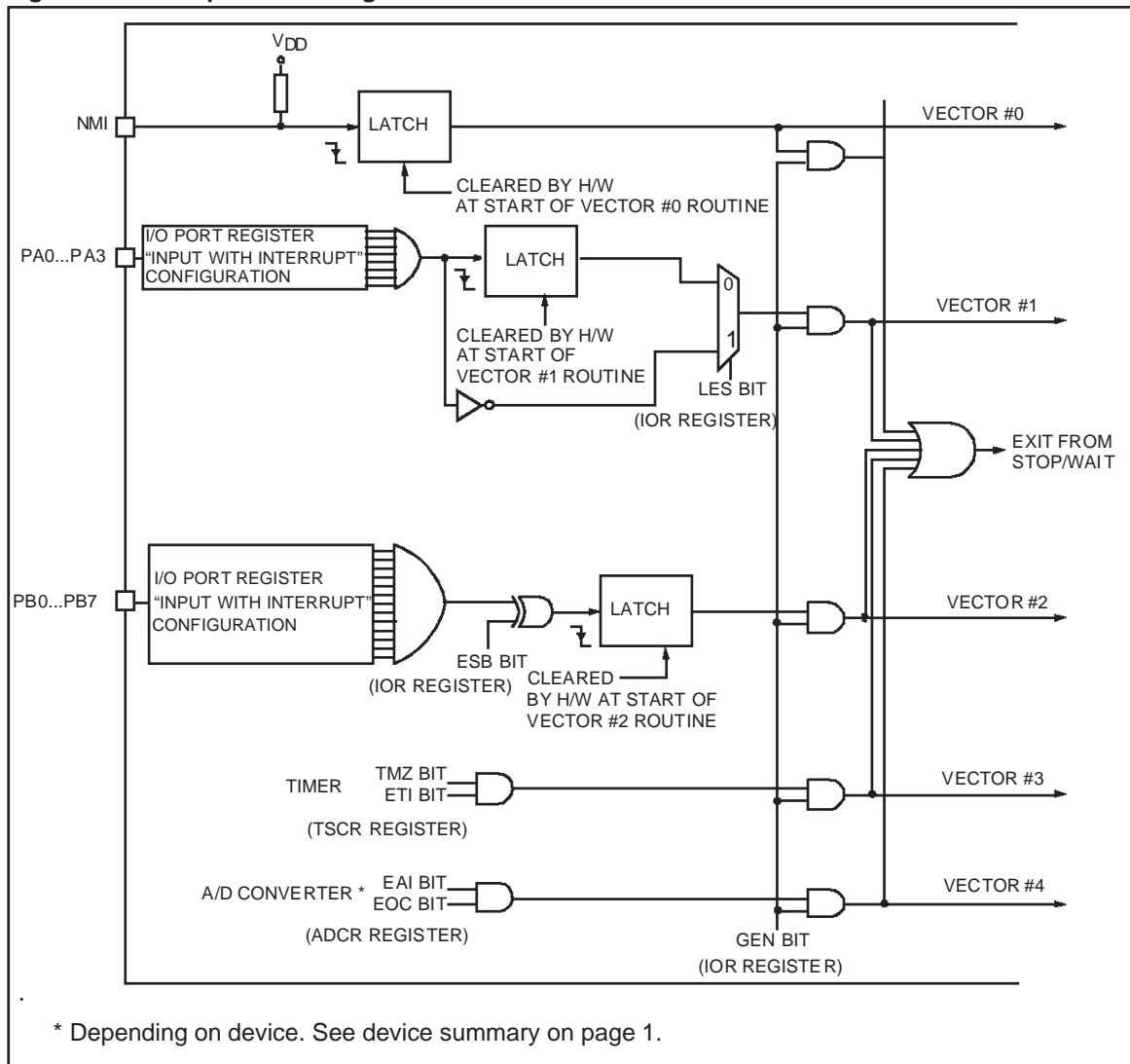
Figure 17. Interrupts Block Diagram
