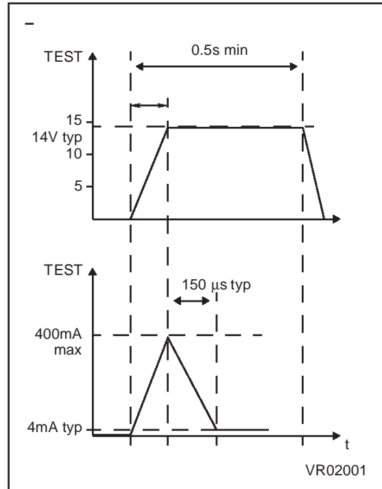
Figure 6. Programming wave form
