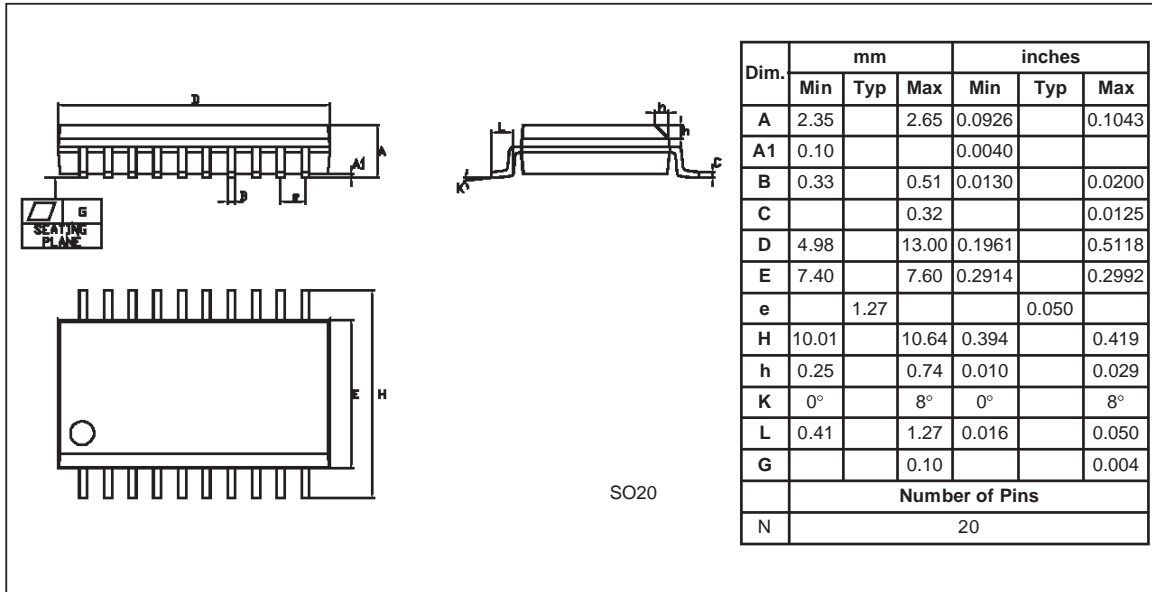
Figure 76. 20-Pin Plastic Small Outline Package, 300-mil Width
