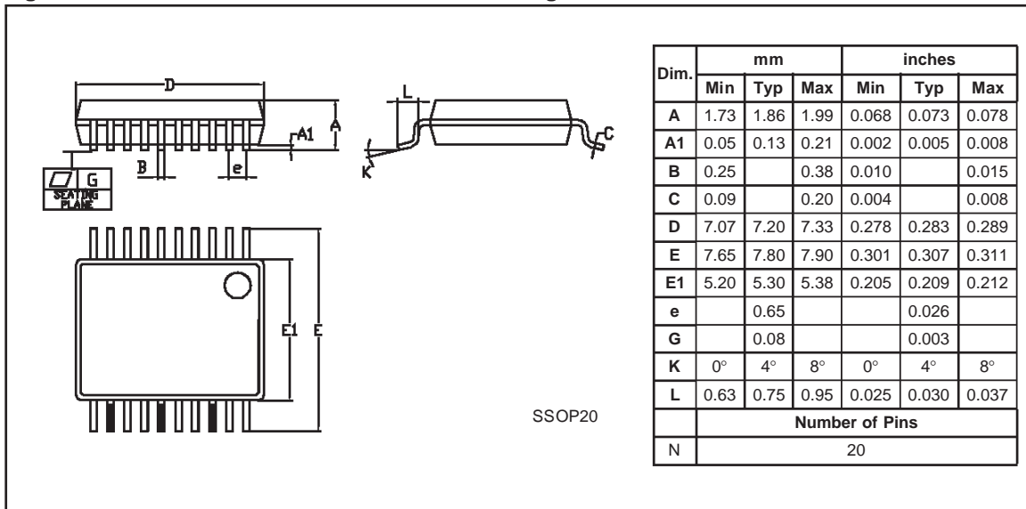
Figure 1. 20-Pin Plastic Shrink Small Outline Package
