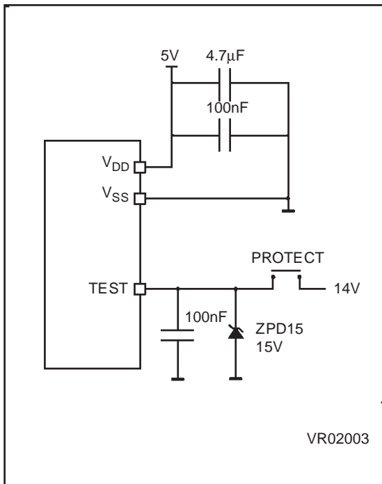
Figure 5. Programming Circuit
