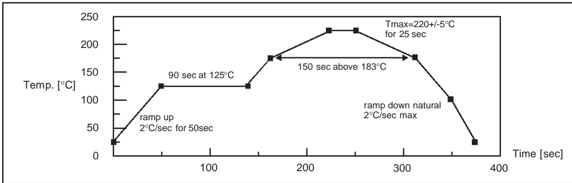
Figure 3. Recommended Reflow Soldering Oven Profile (MID JEDEC)
