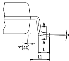
DETAIL "A" (2:1)
