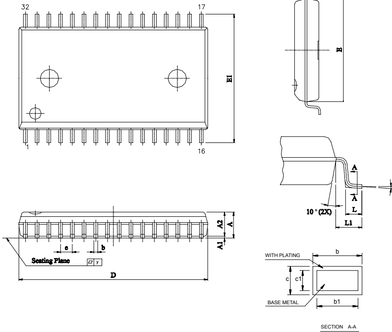
SOP-32
