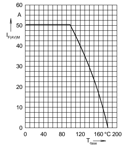
Fig. 5 Max. forward current at case temperature 180° sine
