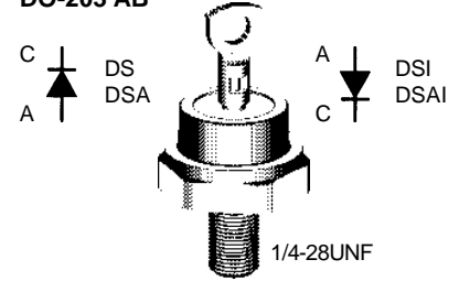
DO-203 AB
