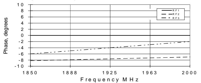
Phase Balance vs. Frequency
