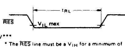
Figure 10 \overline{RES} Low Time
