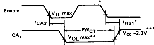
Figure 2 CA 2 Delay Time (Read Mode; CRA5=CRA3=1, CRA4=0)
