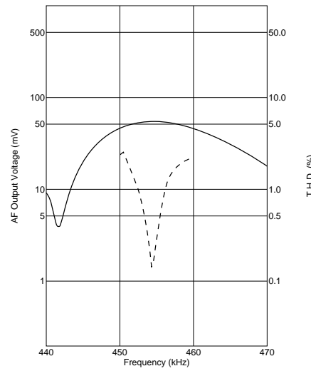
CDBLB455KCAY21-B0
