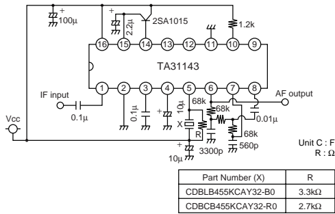
TA31143
