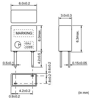
CDBLB_CAX Series
