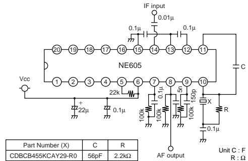
NE605
