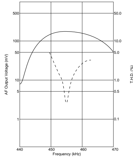
CDBLB455KCAX16-B0
