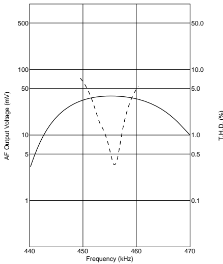
CDBLA/CDBLB455KCAY42-B0
