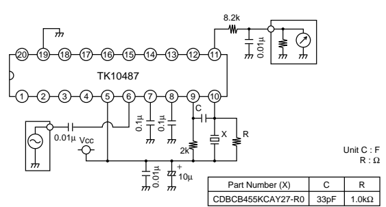
TK10487
