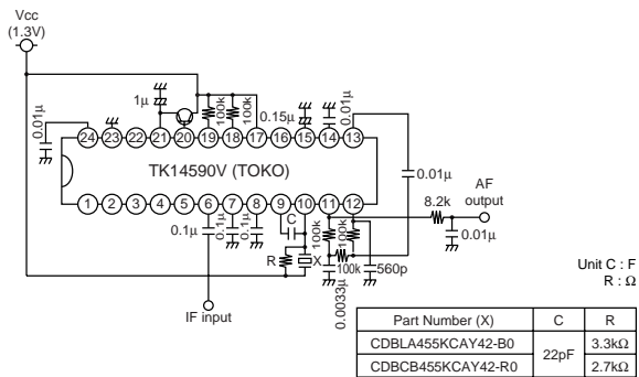
TK14590/14591
