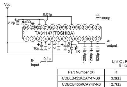
TA31147
