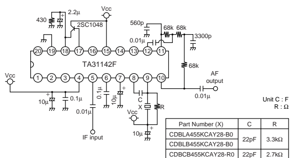
TA31142
