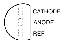
TO-92 PACKAGE (TOP VIEW)
