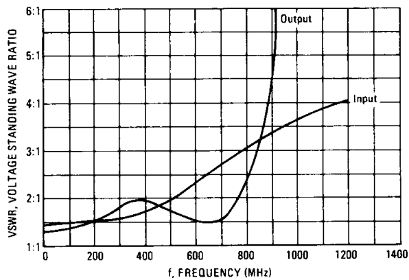
FIGURE 9 – VSWR versus FREQUENCY MWA230
