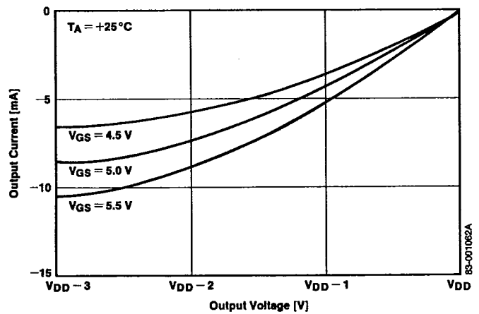
Output Current vs Output Voltage [P-Channel]
