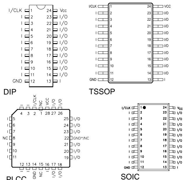
Figure 1. Pin Configuration
