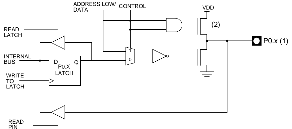
Figure 2. Port 0 Structure
