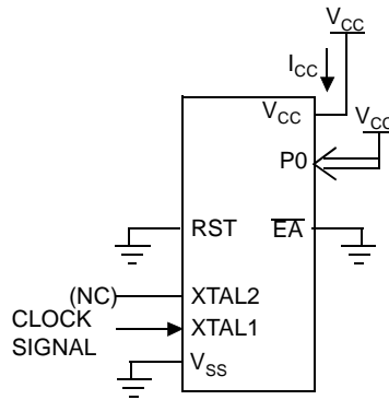
Figure 65. I_{CC} Test Condition, Idle Mode
