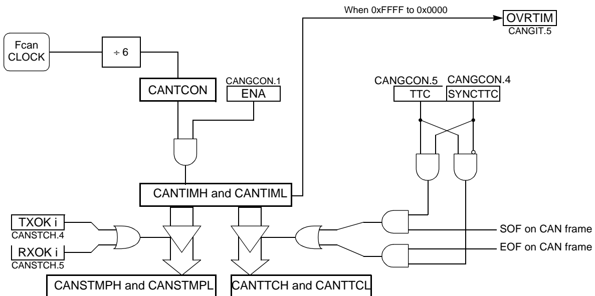
Figure 51. Block Diagram of CAN Timer
