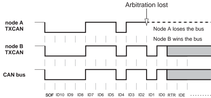
Figure 42. Bus Arbitration
