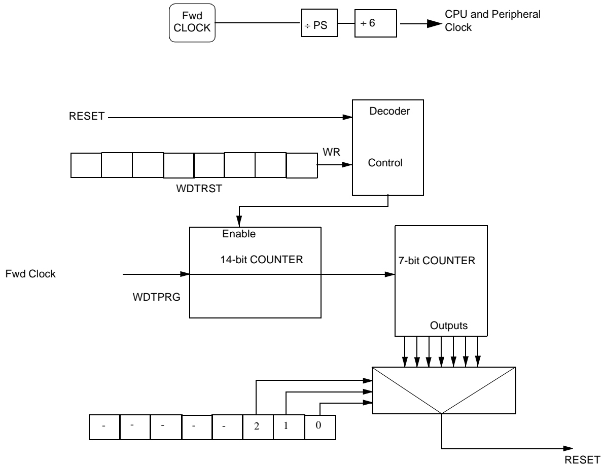
Figure 38. Watchdog Timer
