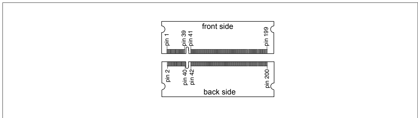
Figure 1 Pin Configuration
