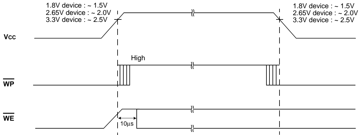
Figure 24. AC Waveforms for Power Transition
