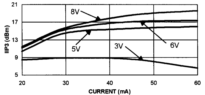
INPUT IP3 vs. CURRENT, F=1785 MHz
