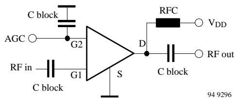
Amplifier 1
